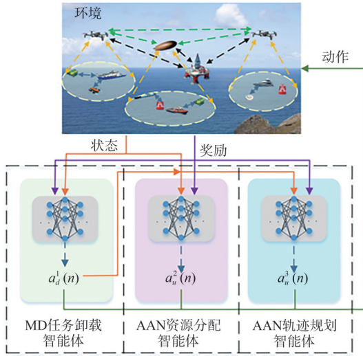
图3 异构多智能体协同优化框架
